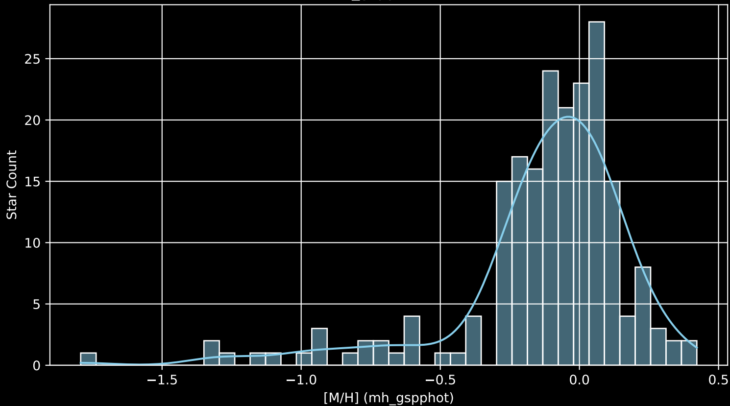
APOGEE DR17 Field: [146-04 [M/H] (mh_gspphot) (n= 204)
